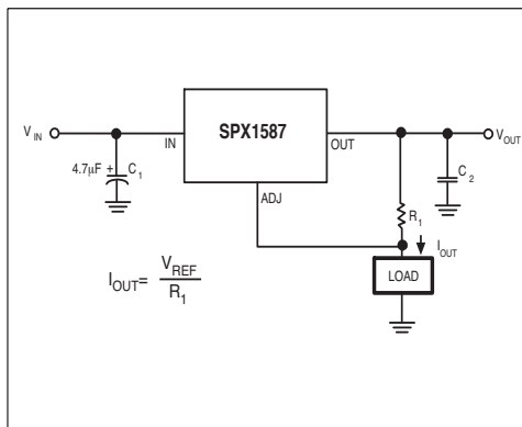
Figure 6. Current Source
