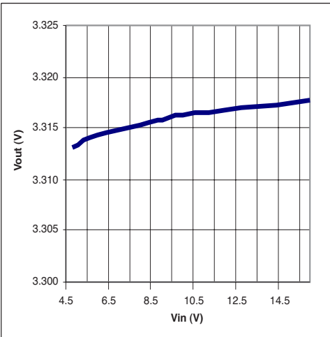
Figure 1. Line Regulation for SPX1587U-3.3; I_{OUT}=10\text{mA}
