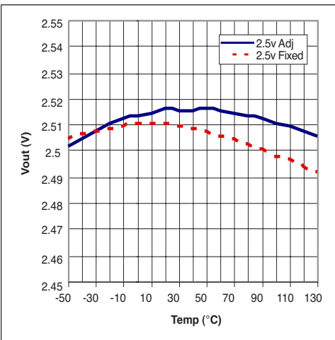
Figure 3. V_{IN}=4.0\text{V} , I_{OUT}=10\text{mA}
