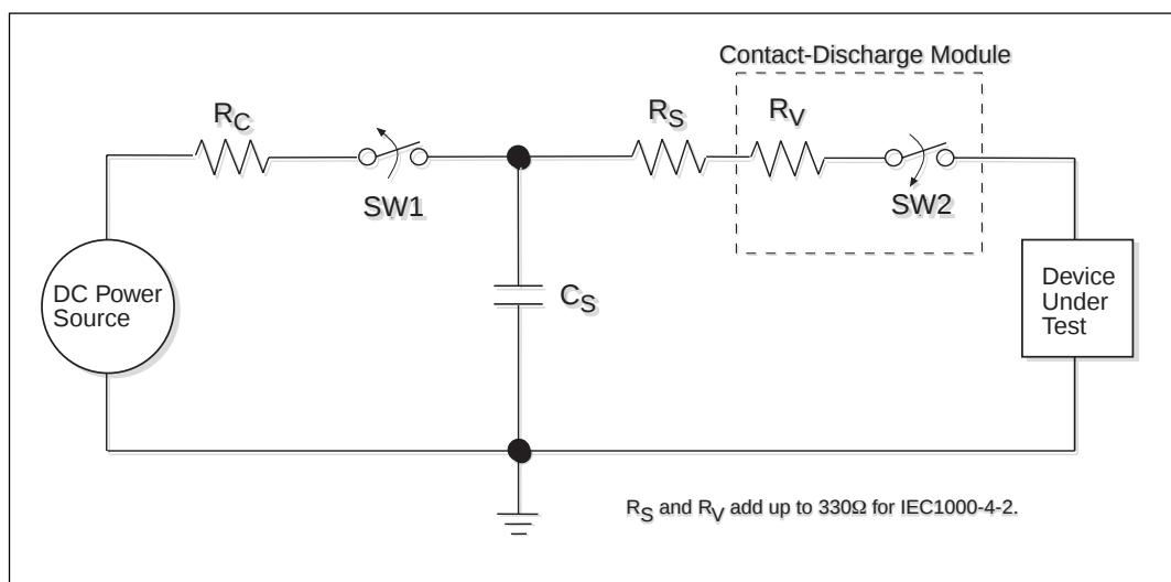
Figure 18. ESD Test Circuit for IEC1000-4-2
