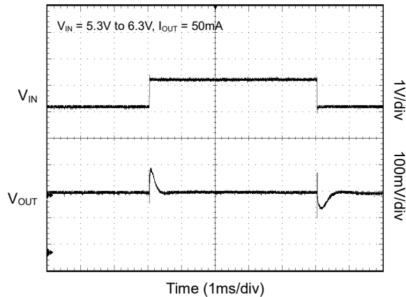
Line-Transient Response
