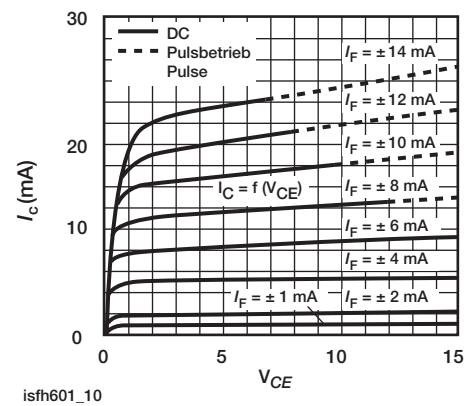
Fig. 10 - Output Characteristics
