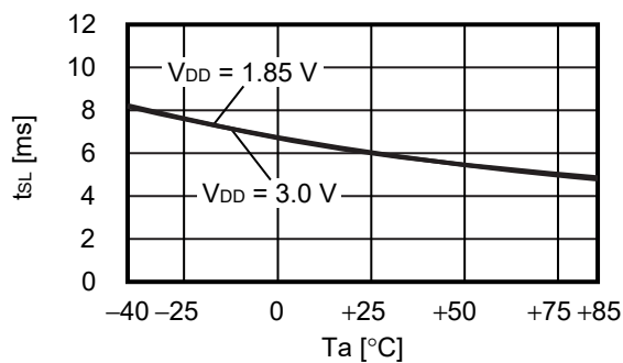
6.7 Sleep mode time ( t_{SL} ) vs. Temperature ( T_a )
