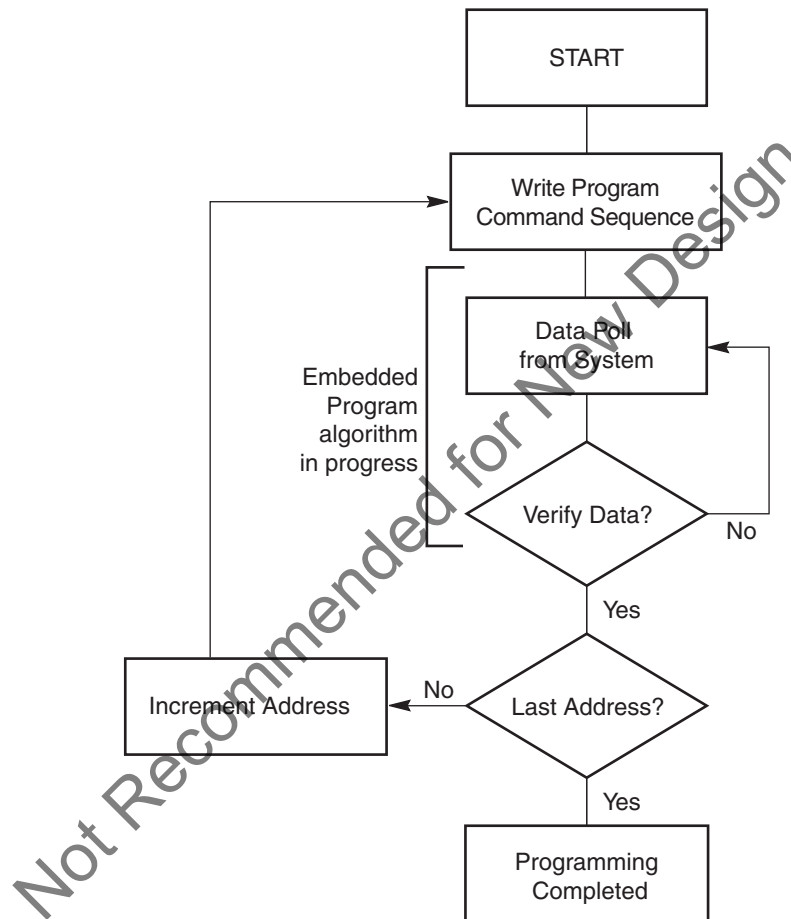
Figure 11.1 Program Operation
