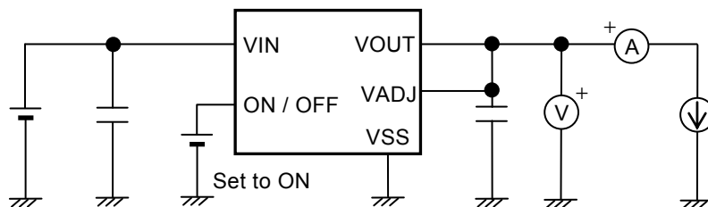
Figure 19 Test Circuit 7
