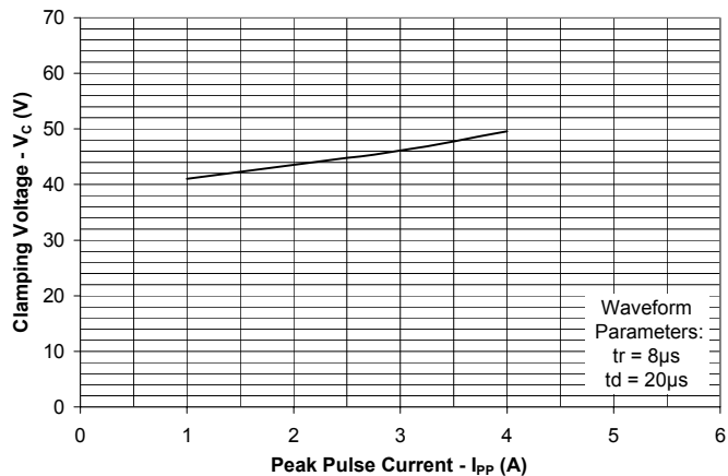
Clamping Voltage vs. Peak Pulse Current (Pin 6 to GND)
