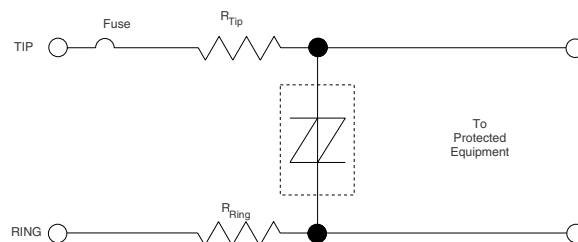
FIGURE 1 - Metallic Protection
