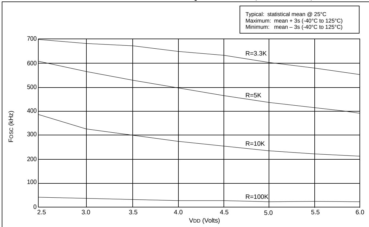
FIGURE 16-4: TYPICAL RC OSCILLATOR FREQUENCY vs. V_{DD} , C_{EXT} = 300 pF, 25^{\circ}\text{C}
