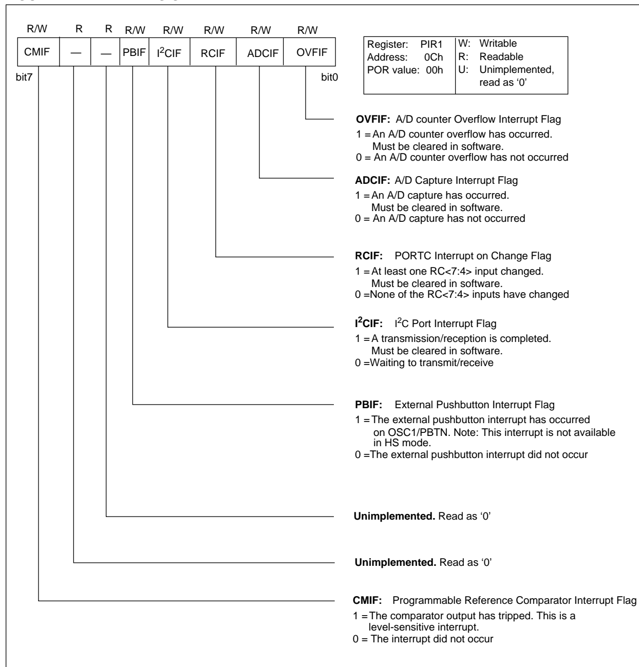
FIGURE 4-7: PIR1 REGISTER
