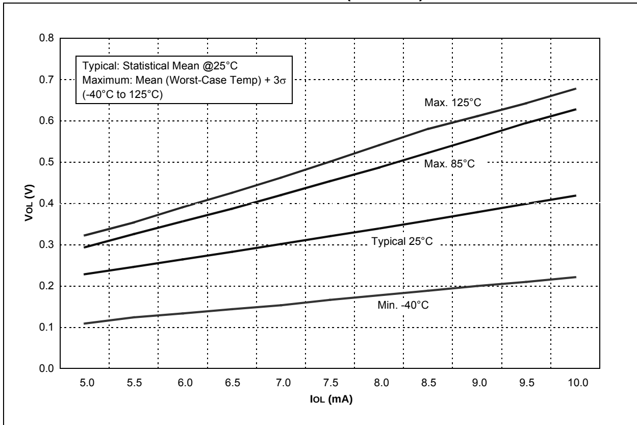
FIGURE 12-9: V OL vs. I OL OVER TEMPERATURE (V DD = 3.0V)
