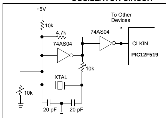
FIGURE 8-3: EXTERNAL PARALLEL RESONANT CRYSTAL OSCILLATOR CIRCUIT
