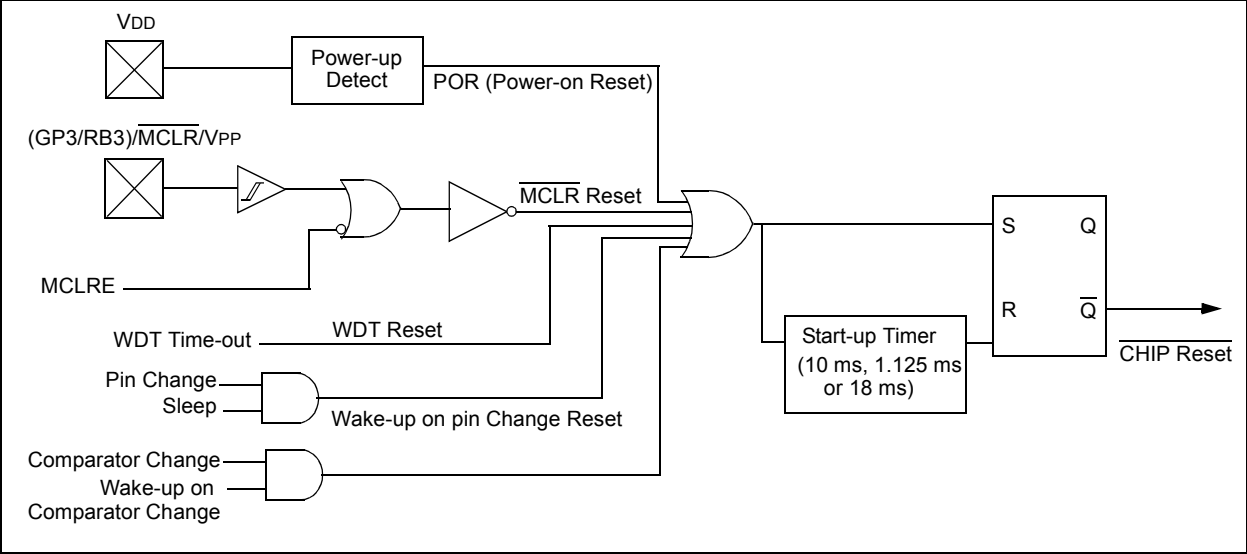
FIGURE 10-8: TIME-OUT SEQUENCE ON POWER-UP ( \overline{\text{MCLR}} PULLED LOW)
