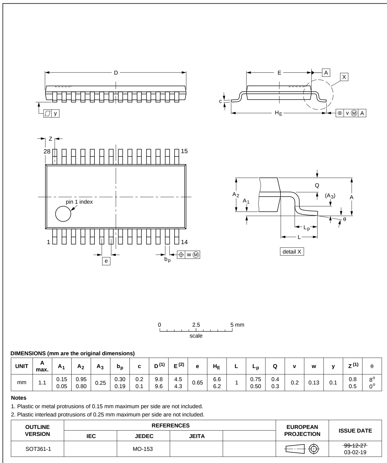
Fig 23. Package outline SOT361-1 (TSSOP28)
