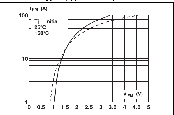
Figure 8. Peak forward voltage drop vs. peak forward current for unidirectional types (typical value). (1)
