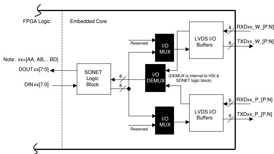
Figure 2. ORT8850 Embedded Core, Top Level Functionality and Data Flow
