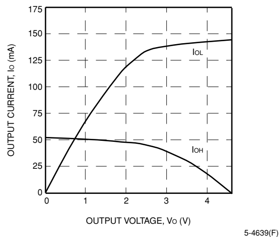
Figure 82. Fast ( T_J = 125^\circ\text{C} , V_{DD} = 4.5\text{ V} )
