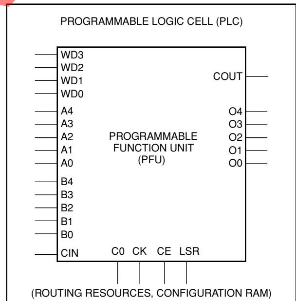
Figure 2. PFU Ports
