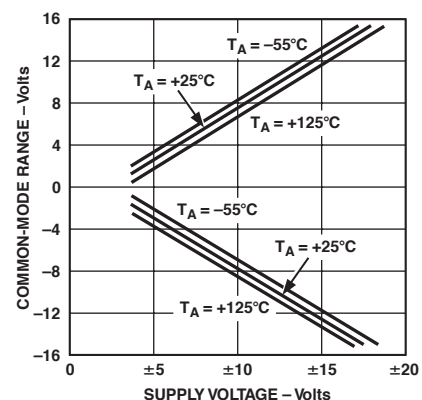
TPC 27. Common-Mode Input Range vs. Supply Voltage
