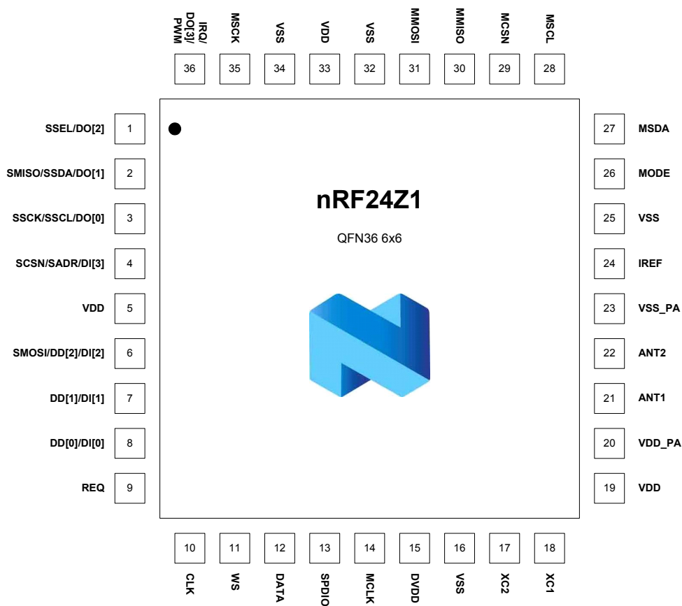
Figure 1. Pin assignments
