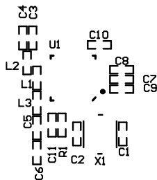
Top silk screen
