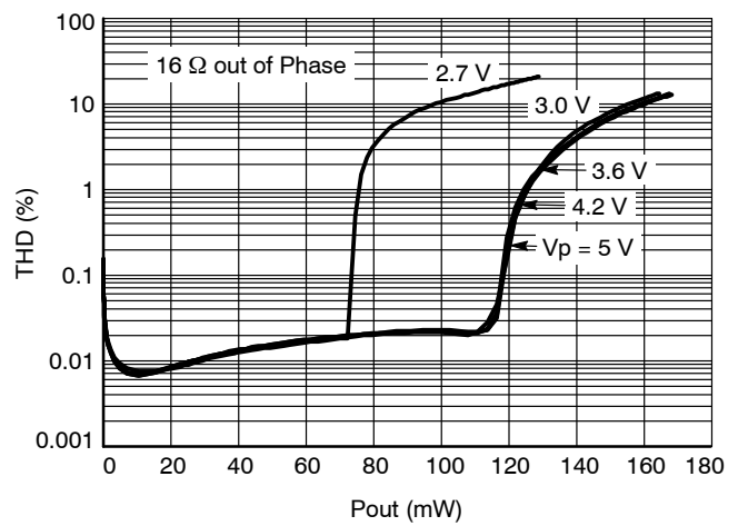
Figure 10. THD+N vs. Pout RIGHT
