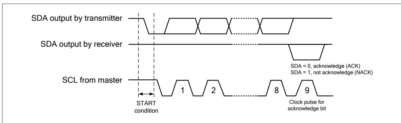
Figure 15.1-5. Acknowledge Bit
