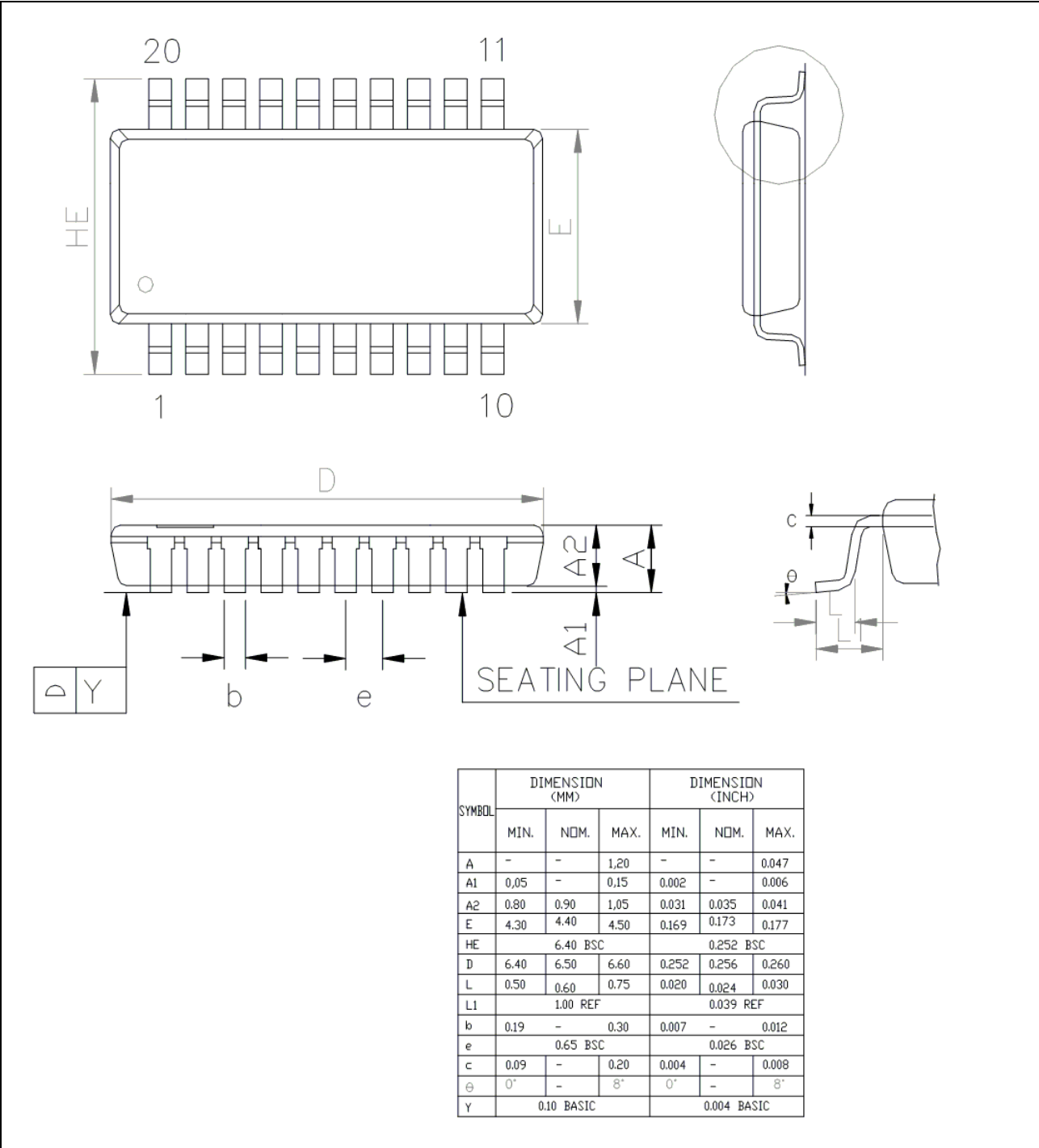
Figure 32.1-1. TSSOP-20 Package Dimension
