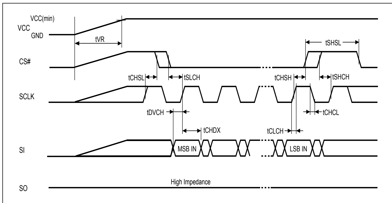
Figure 88. AC Timing at Device Power-Up
