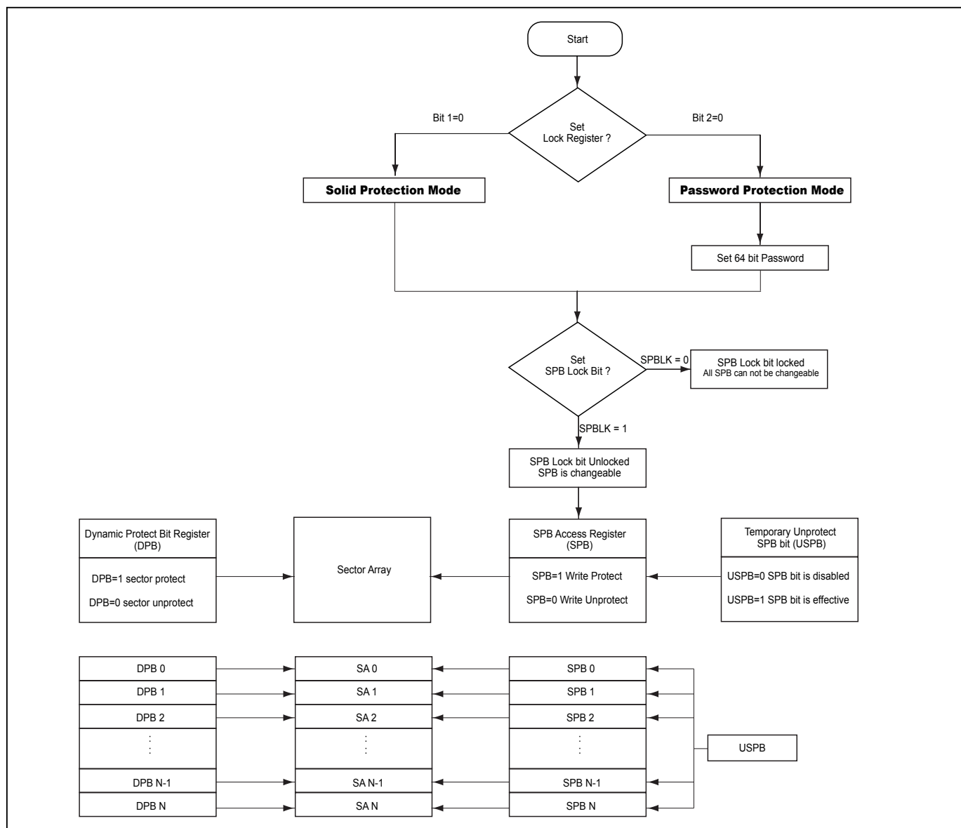
Figure 65. Advanced Sector Protection Overview
