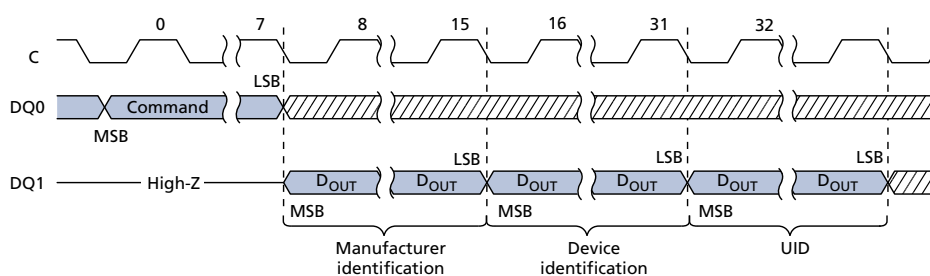
Figure 16: READ ID and MULTIPLE I/O READ ID Commands
