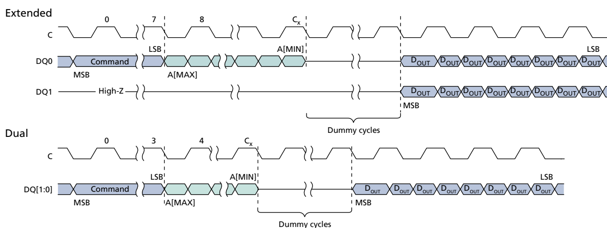
Figure 29: DTR DUAL OUTPUT FAST READ – 3Dh
