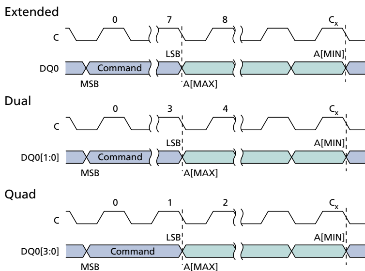
Figure 40: SUBSECTOR and SECTOR ERASE Timing
