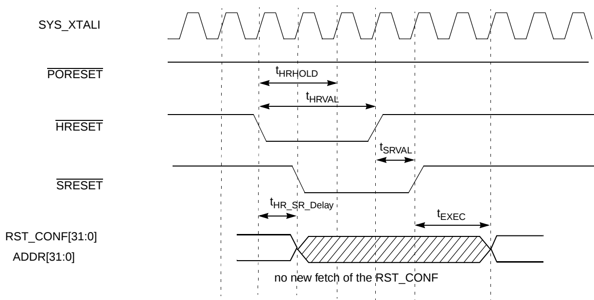
Figure 6. HRESET Behavior
