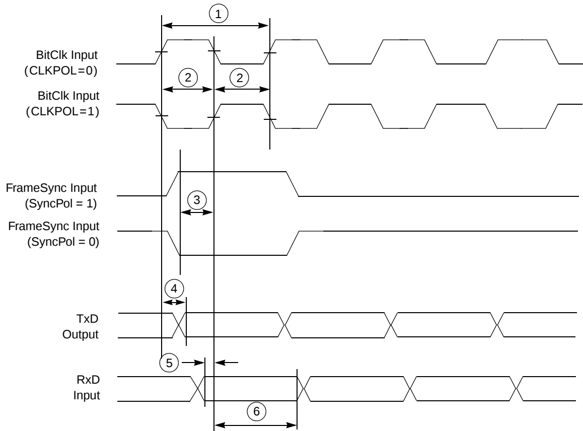
Figure 48. Timing Diagram – 8,16, 24, and 32-bit CODEC/I²S Slave Mode
