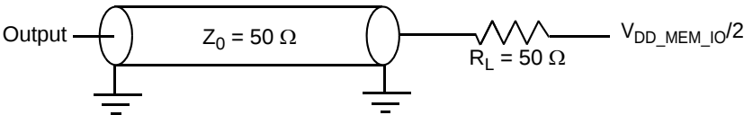
Figure 11. DDR AC Test Load
