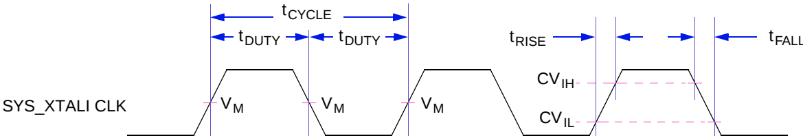
Figure 3. Timing Diagram—SYS_XTALI
