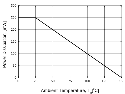
Figure 6. Power Derating
