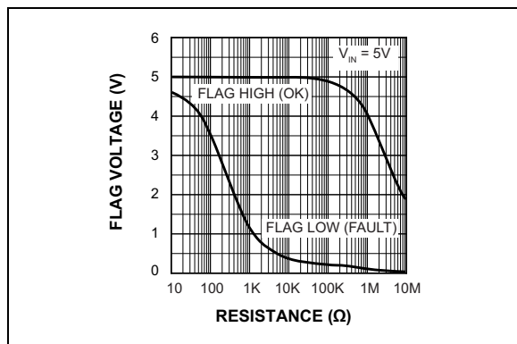
FIGURE 2-19: Error Flag Voltage vs. Pull-Up Resistor Value.
