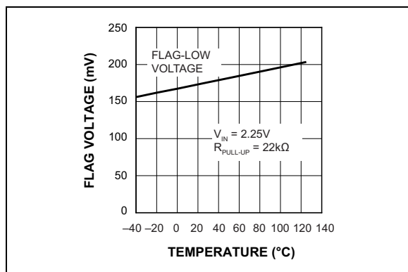
FIGURE 2-21: Flag-Low Voltage vs. Temperature.
