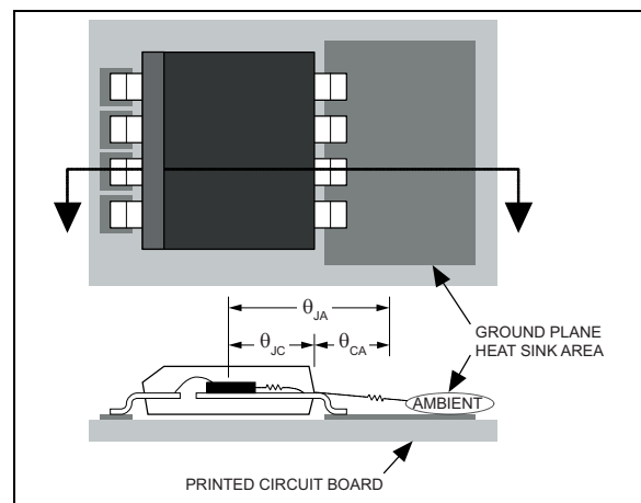
FIGURE 4-3: Thermal Resistance.
