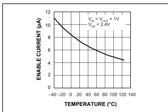
FIGURE 2-20: Enable Current vs. Temperature.
