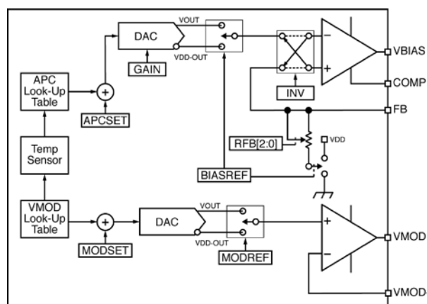
Figure 4. MIC3001 APC and Modulation Control Block Diagram
