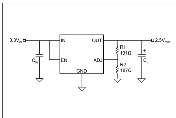
FIGURE 2-27: MIC29302A Load Transient Response Test Circuit.
