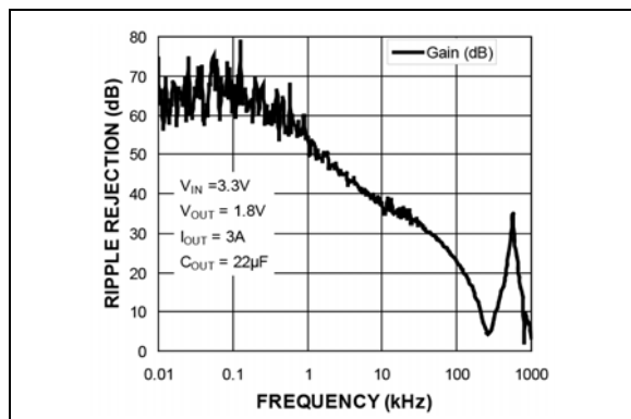
FIGURE 2-25: Ripple Rejection ( I_{OUT} = 3A ) vs. Frequency.
