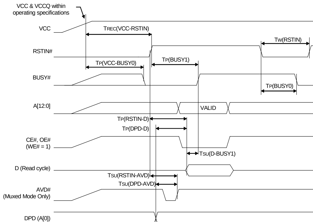
Figure 25: Reset Timing
