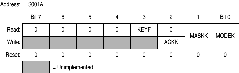
Figure 14-3. Keyboard Status and Control Register (KBSCR)
