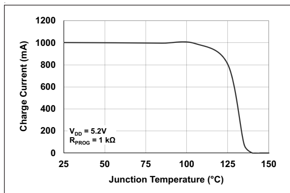
FIGURE 4-3: Thermal Regulation.
