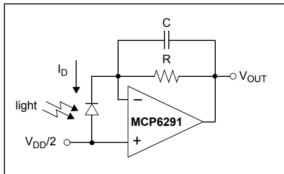
FIGURE 4-9: Photodiode Amplifier.
