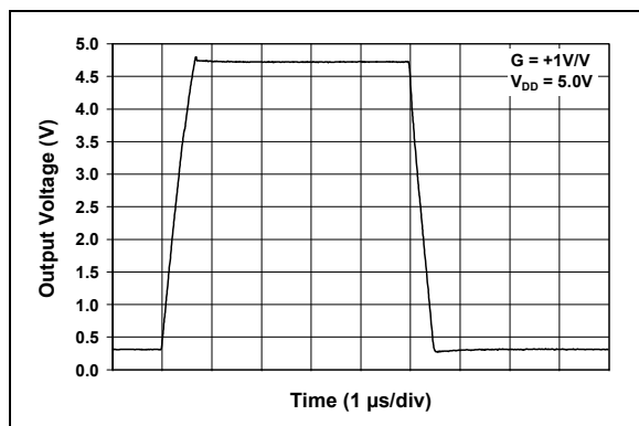
FIGURE 2-25: Large-Signal Noninverting Pulse Response.
