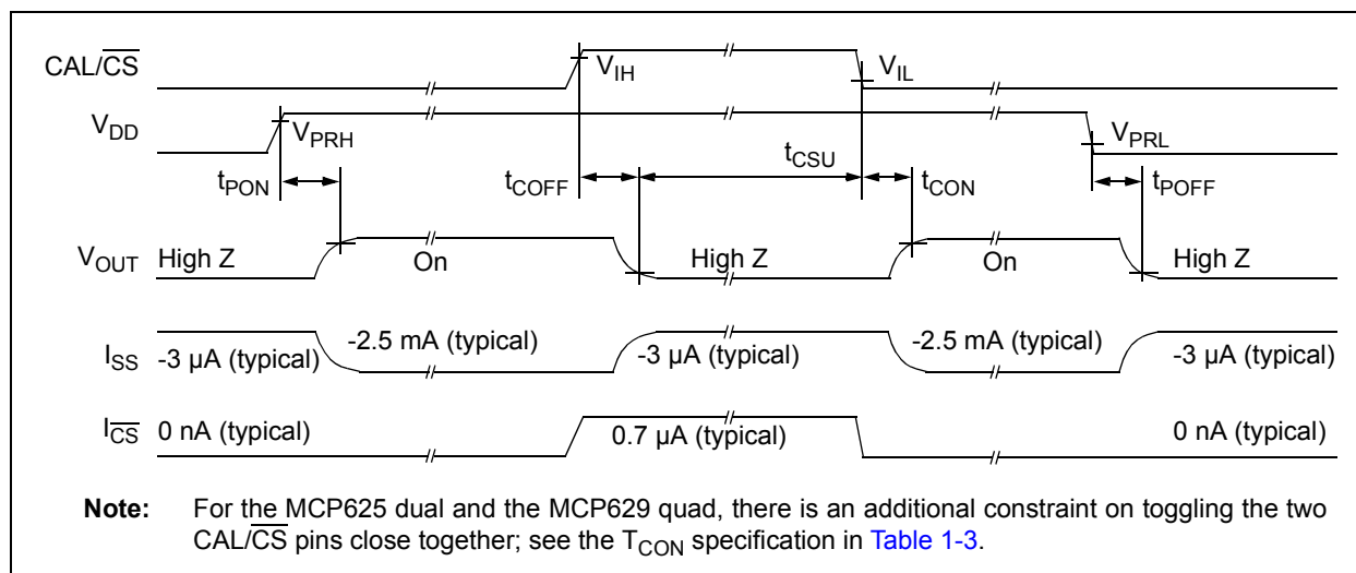
FIGURE 1-1: Timing Diagram.
