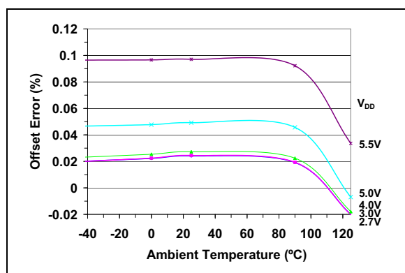
FIGURE 2-20: Offset Error vs. Ambient Temperature and V_{DD} .
