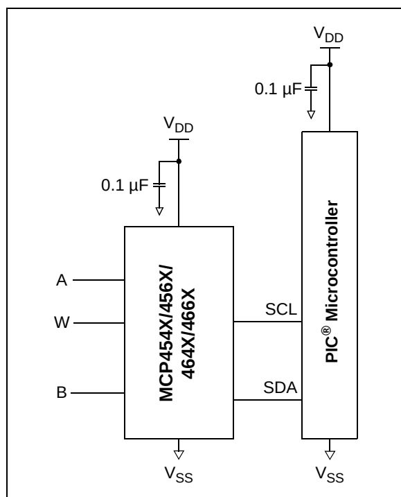
FIGURE 8-6: Typical Microcontroller Connections.
