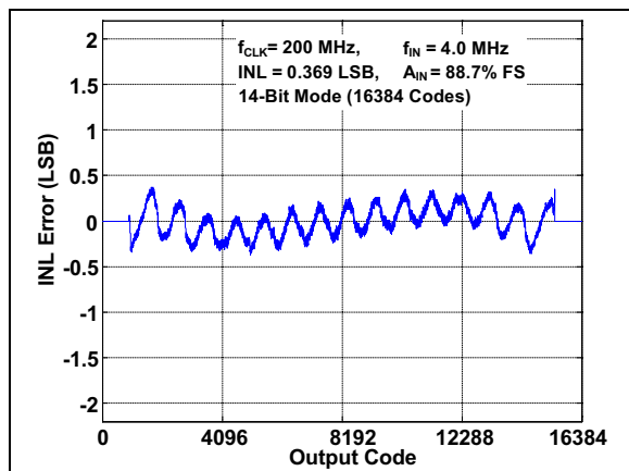
FIGURE 3-30: INL Error Vs. Output Code: f_S = 200 \text{ Mps} , f_{IN} = 4 \text{ MHz} , 14-bit Mode.
