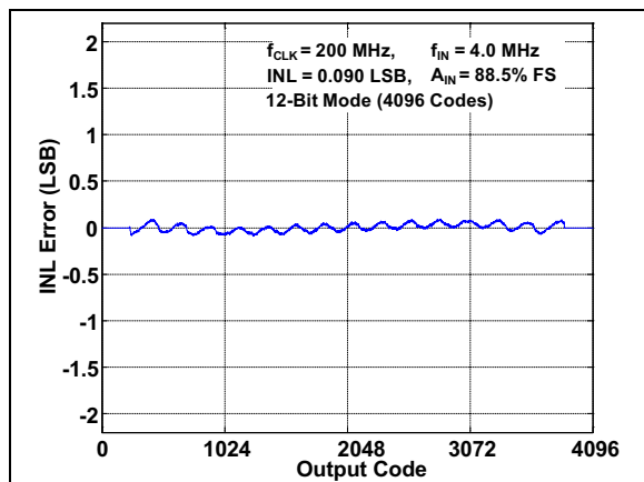
FIGURE 3-31: INL Error Vs. Output Code: f_S = 200 \text{ Mps} , f_{IN} = 4 \text{ MHz} , 12-bit Mode.
