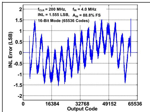
FIGURE 3-29: INL Error Vs. Output Code: f_S = 200 \text{ Mps} , f_{IN} = 4 \text{ MHz} , 16-bit Mode.
