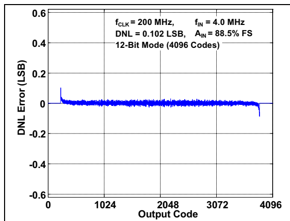
FIGURE 3-34: DNL Error Vs. Output Code: f_S = 200 \text{ Mps} , f_{IN} = 4 \text{ MHz} , 12-bit Mode.
