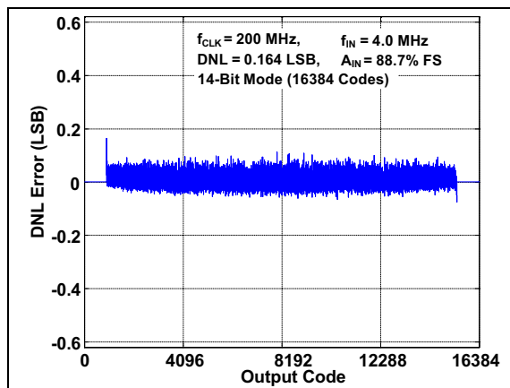
FIGURE 3-33: DNL Error Vs. Output Code: f_S = 200 \text{ Mps} , f_{IN} = 4 \text{ MHz} , 14-bit Mode.
