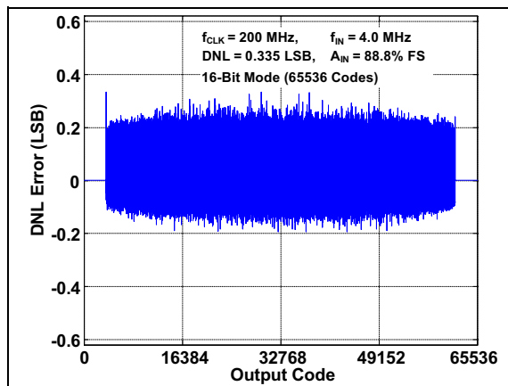
FIGURE 3-32: DNL Error Vs. Output Code: f_S = 200 \text{ Mps} , f_{IN} = 4 \text{ MHz} , 16-bit Mode.
