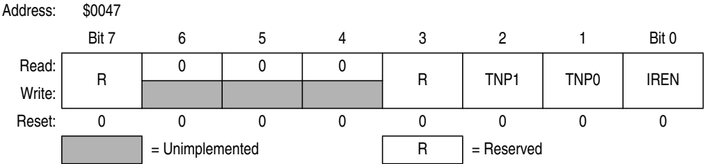
Figure 12-20. IRSCI Infrared Control Register (IRSCIRCR)
