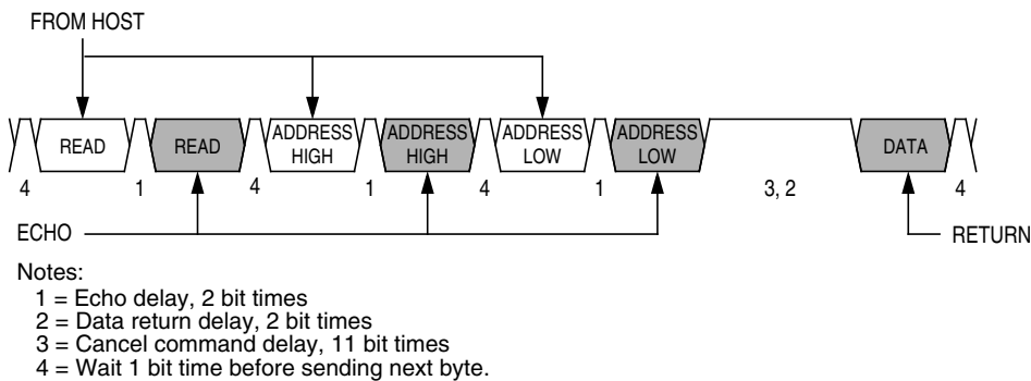
Figure 8-5. Read Transaction
