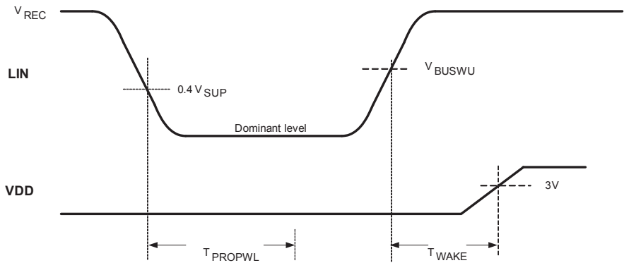
Figure 16. LIN Wake-up LP V_{DD} OFF Mode Timing
