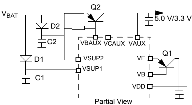
Partial View ex2: Split V_{SUP} Supply
