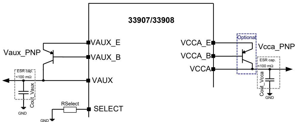
Figure 59. Vaux/VCCA connection
