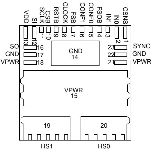
Figure 3. 10XSD200 Pin Assignments
