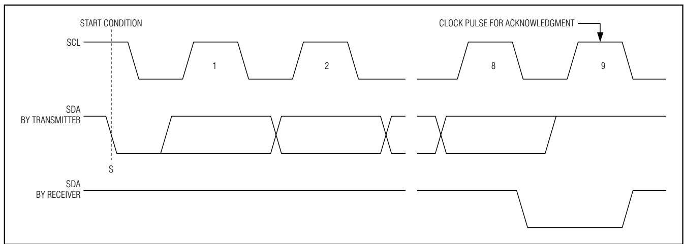
Figure 5. Acknowledge
