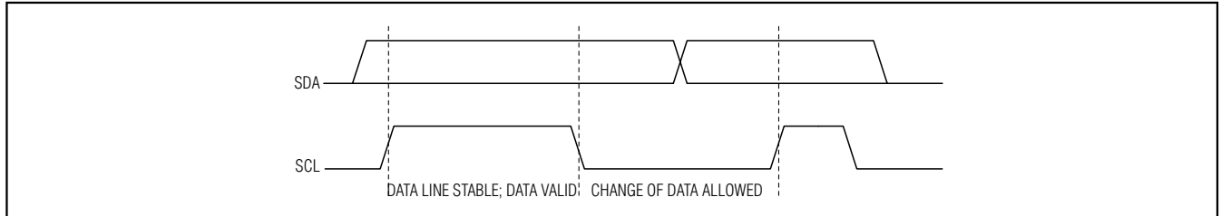
Figure 4. Bit Transfer
