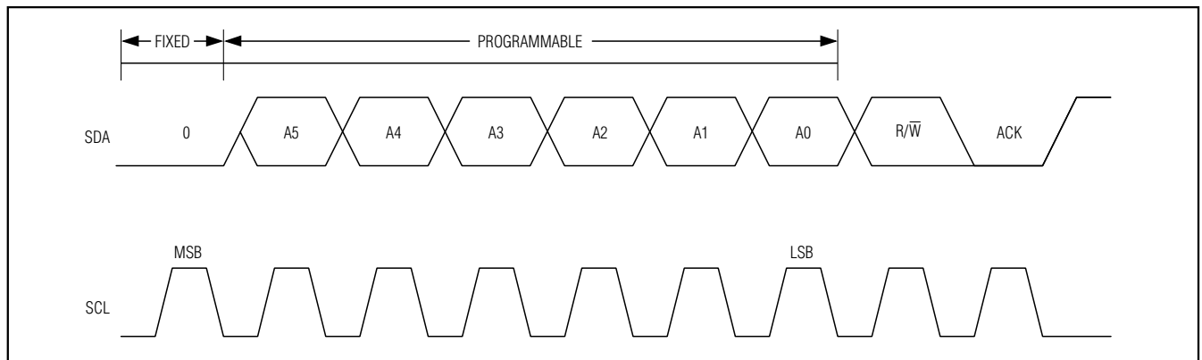
Figure 6. Slave Address
