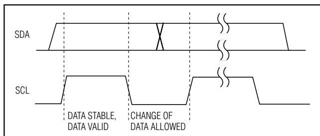
Figure 4. Bit Transfer
