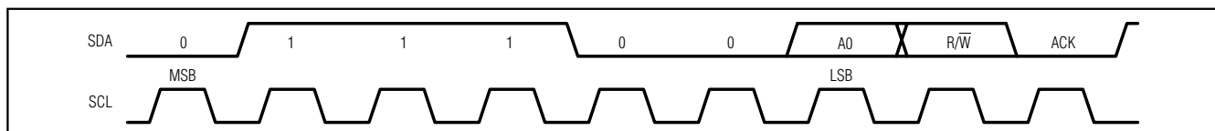
Figure 3. Slave Address
