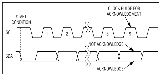
Figure 5. Acknowledge
