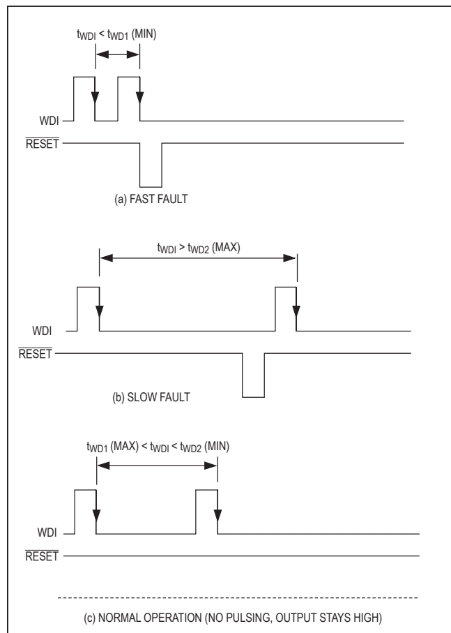
Figure 5. MAX6752/MAX6753 Window Watchdog Diagram
