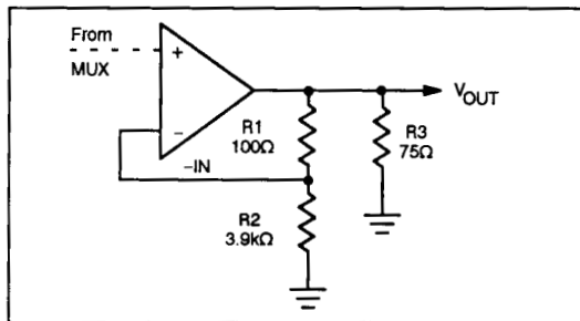
Figure 2. Unity-Gain Connections
