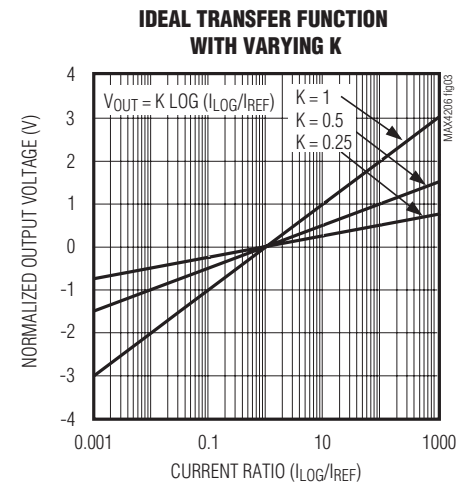
Figure 3. Ideal Transfer Function with Varying K
