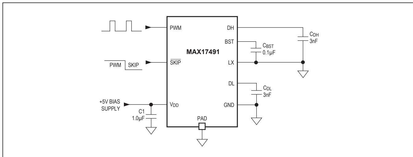
Figure 1. Test Circuit
