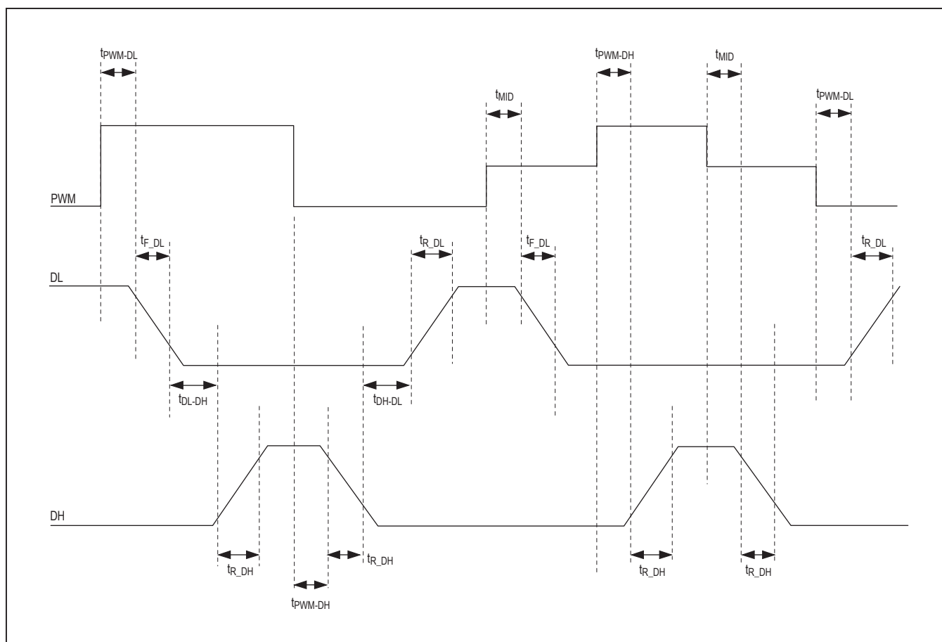
Figure 2. Timing Diagram
