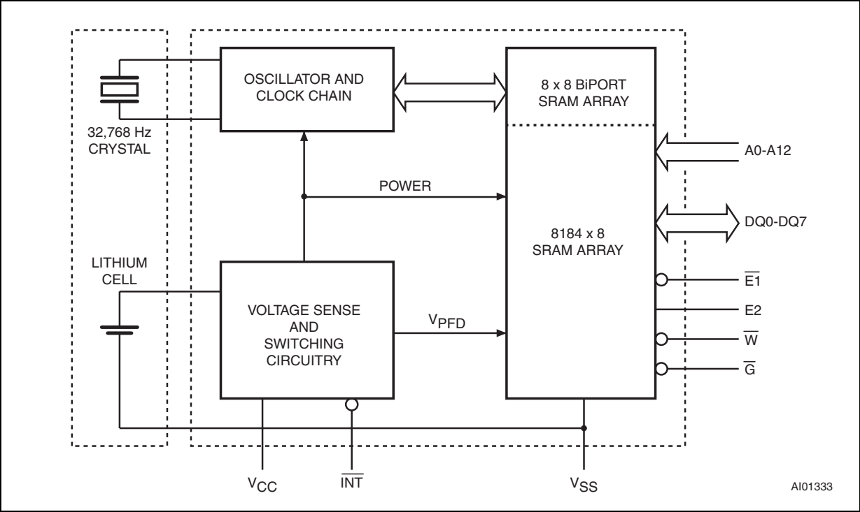
Figure 4. Block diagram
